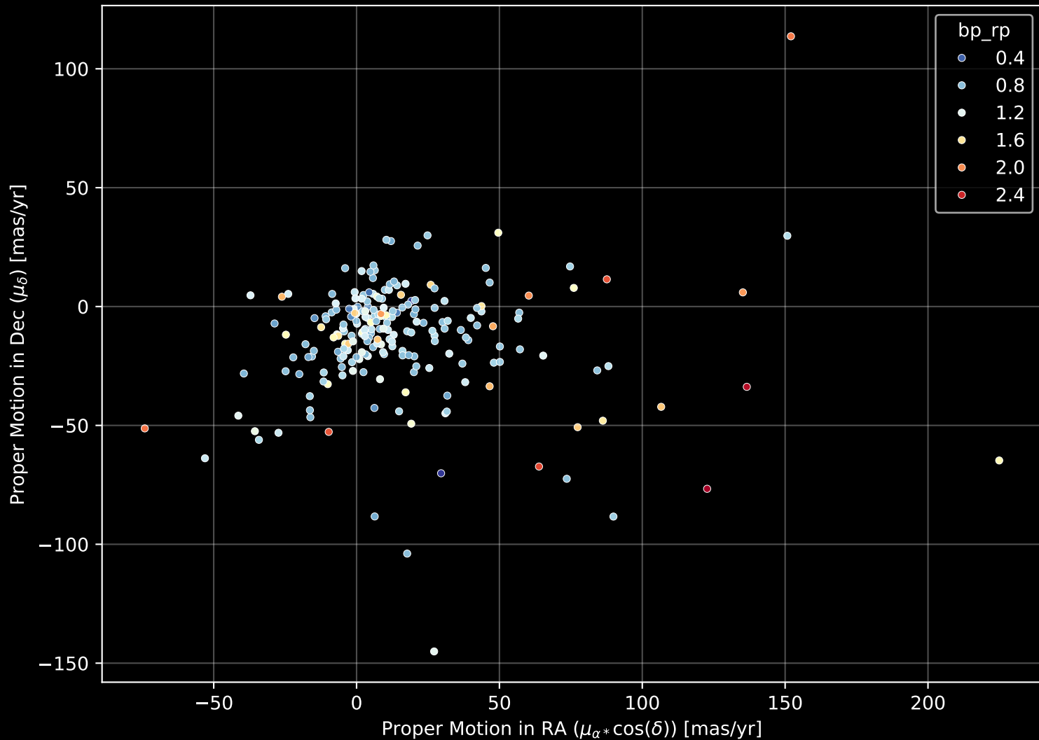
APOGEE DR17 Field: [156-59_MGA] Proper Motion Diagram (n= 217)
