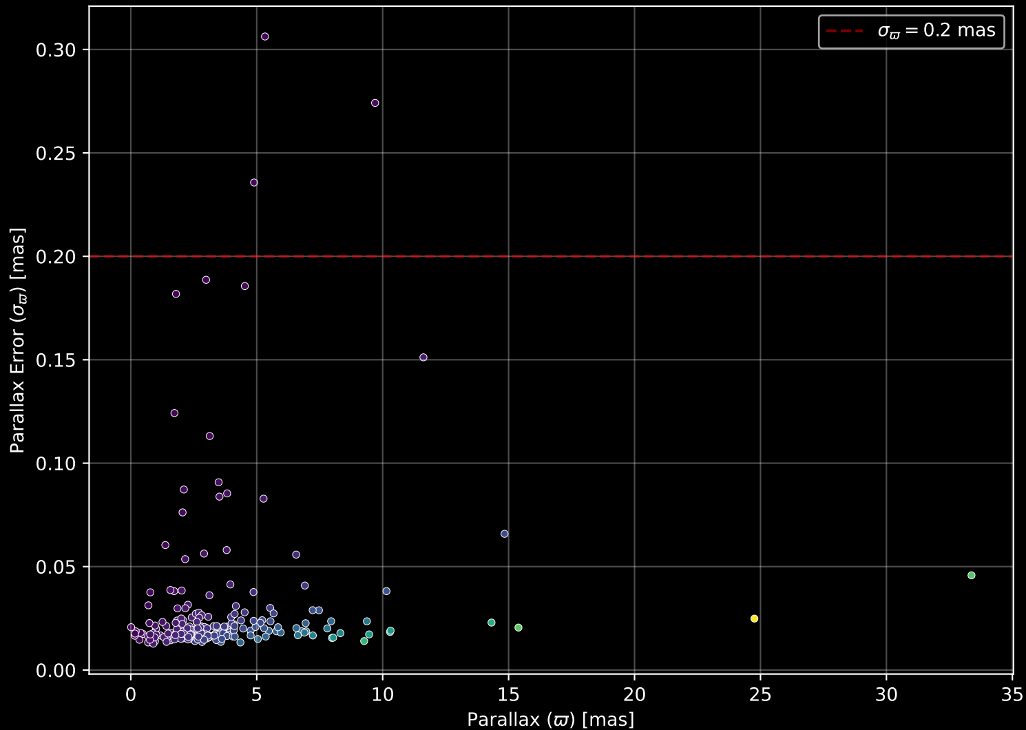
APOGEE DR17 Field: [156-59_MGA] Parallax Quality (n= 217)
