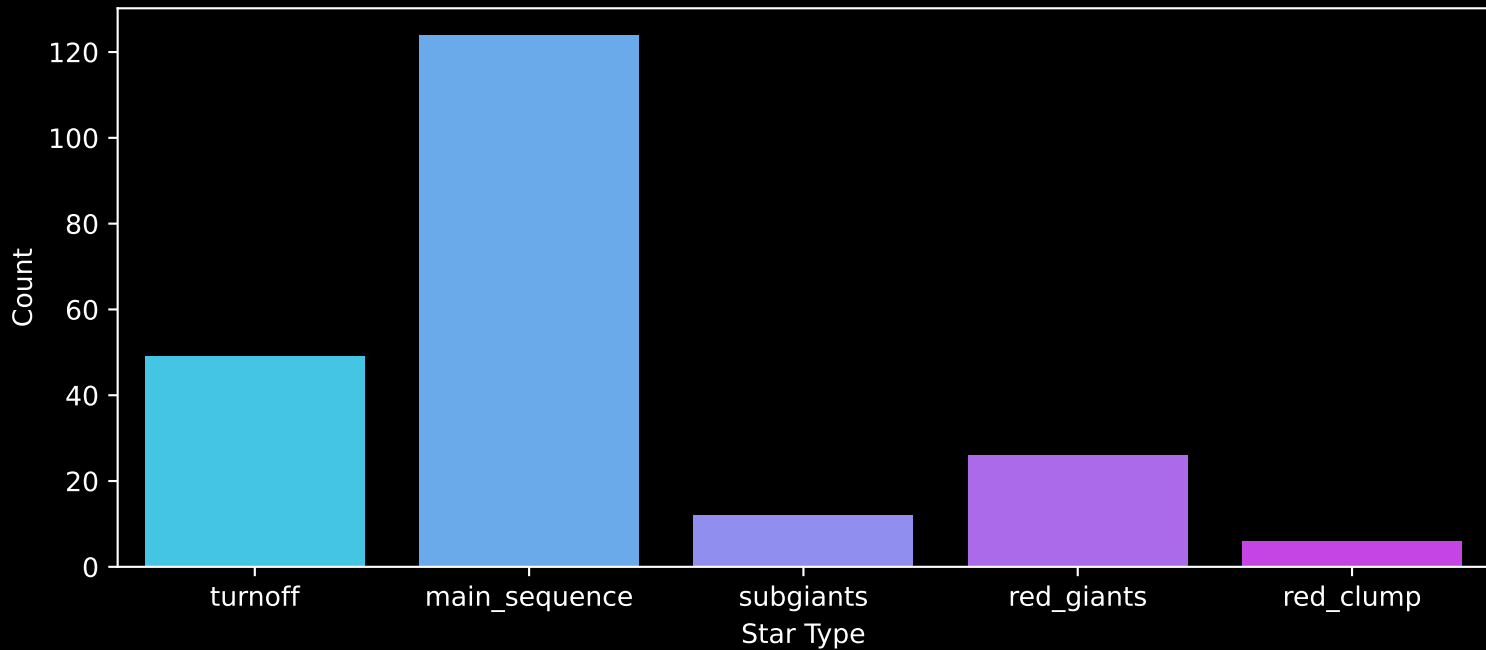
APOGEE DR17 Field: [156-59_MGA] Count plot of Star Type
