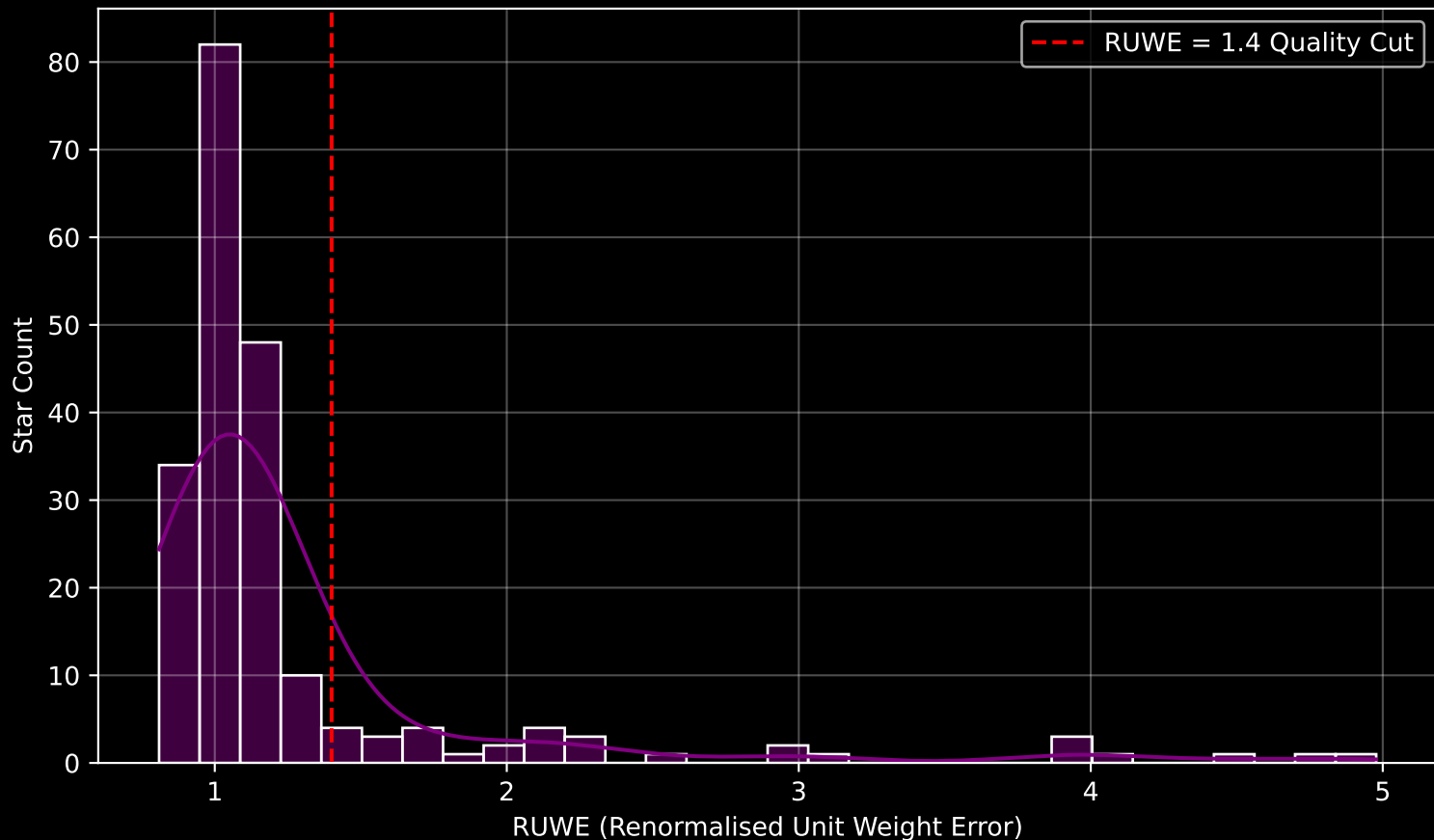
GAPOGEE DR17 Field [156-59_MGA] RUWE Distribution (n= 206)
