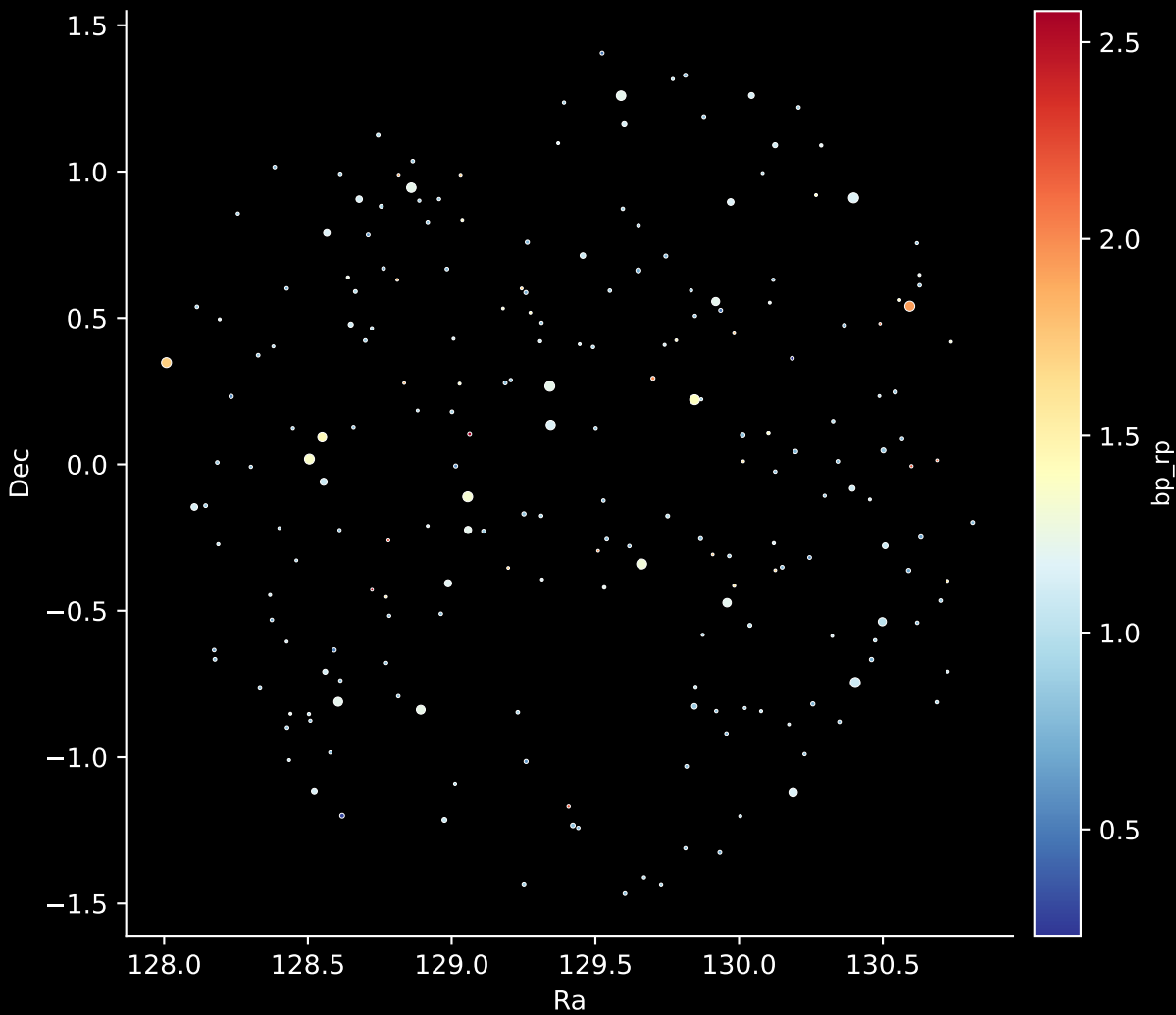
APOGEE DR17 Field: [156-59_MGA] Stars: 217
