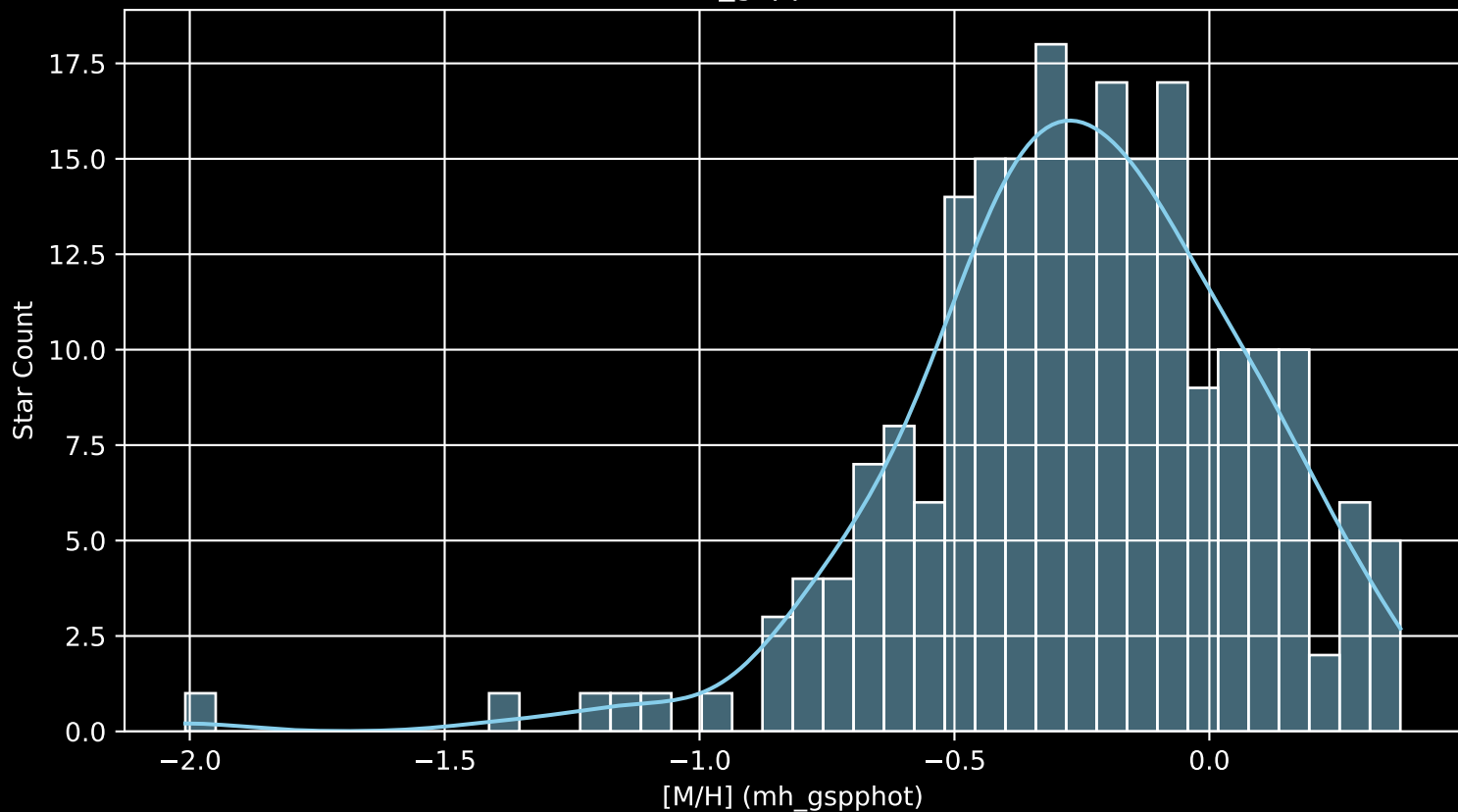
APOGEE DR17 Field: [156-59_MGA [M/H] (mh_gspphot) (n= 216)
